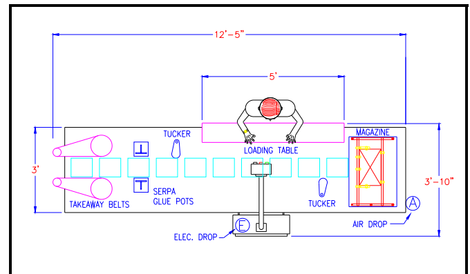
STANDARD RANGE FLOOR PLAN SHOWN
