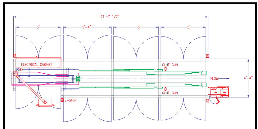
STANDARD RANGE FLOOR PLAN SHOWN
