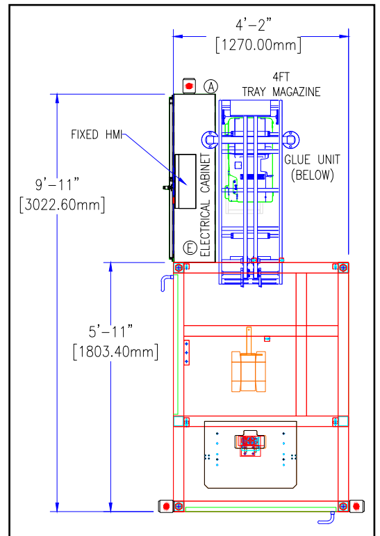
Standard Range Floorplan
