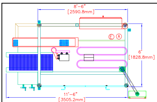
Standard Range Floorplan
